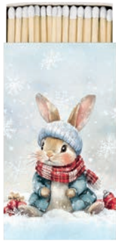
39520980 Buggy Matches
